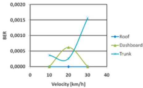
Fig. 10. Study of the antenna location relative to BER
