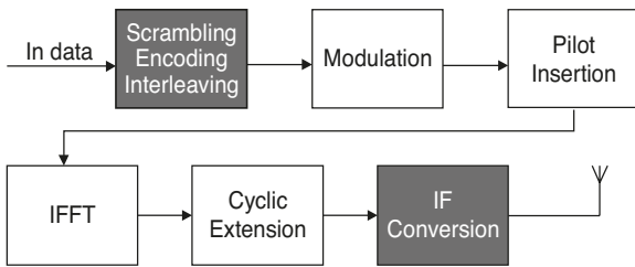
Fig. 4. The OFDM Transmission Operations/Blocks: Modulation, Pilot Insertion, IFFT and Cyclic Extension.
