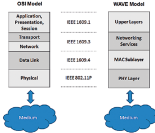
Fig. 2. OSI/WAVE protocol stacks mapping.
