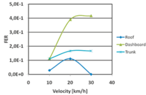
Fig. 11. Study of the antenna location relative to FER
