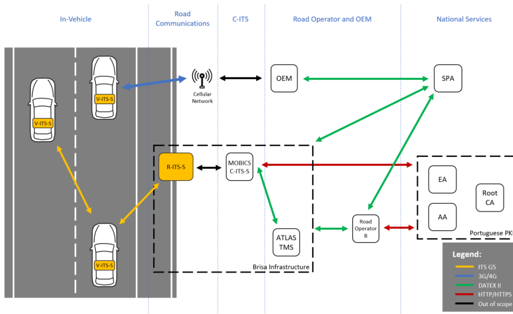
Figure 5 – A-to-Be’s C-ITS architecture
