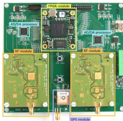
Figure 8 – Radio and interfaces board [4]
