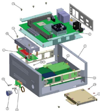
Figure 7 – A-to-Be ITS station hardware
